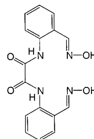
Fig. 1 Chemical structure of \text{H}_4\text{L} .
